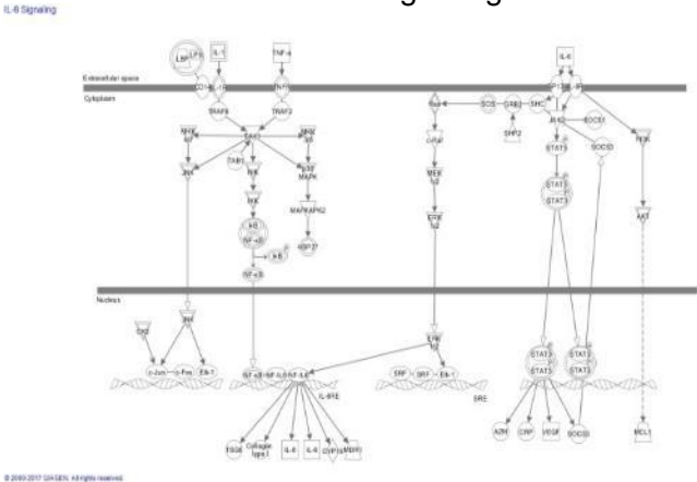
IL6 Signaling
